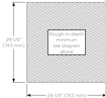
Rough-in Dimensions
