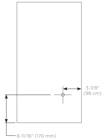
Back of Cabinet - Wire Access Location
