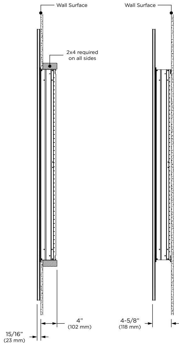
Recessed Mount
