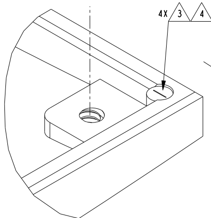
DETAIL A SCALE 1.500
