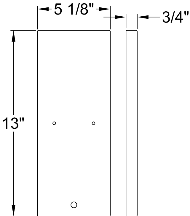
Back Plate
