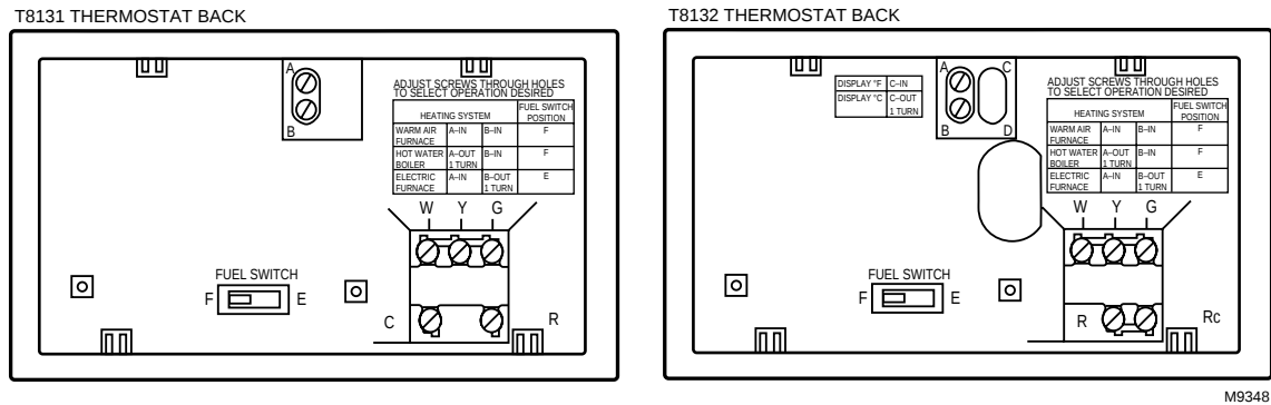
Fig. 12—T8131 and T8132 back.
