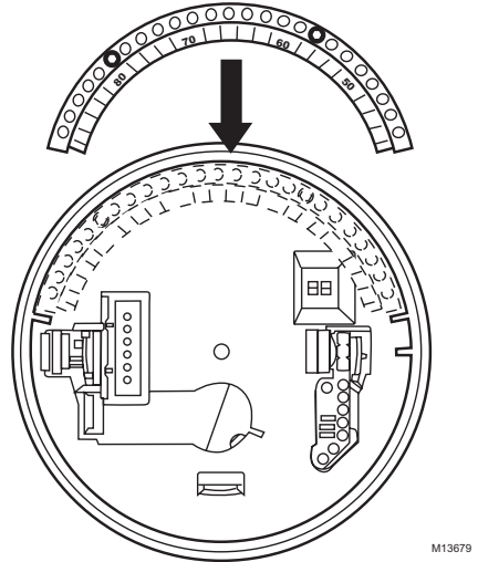
Fig. 3. Aligning range stop with thermostat.
