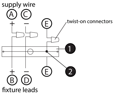
Drawing 3 - Post-Mount
