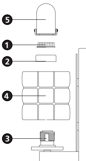
Drawing 2 - Fixture Assembly
