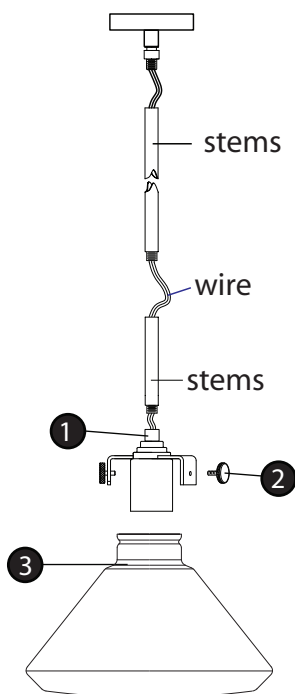
Drawing 3 - Glass Installation
