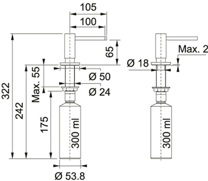
Technical Drawing
