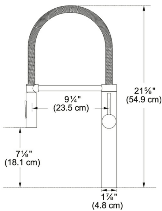
Technical Drawing
