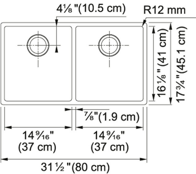
Technical Drawing
