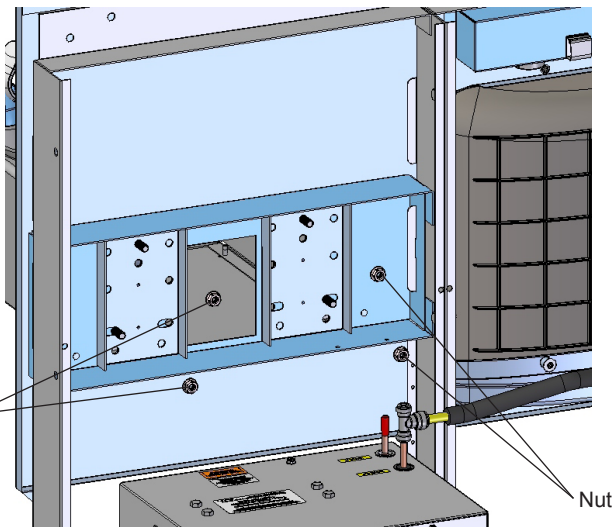
Figure 7 – Fountain Installation
