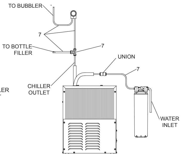
Figure 6 – LZWS-ERFP Tube Routing
