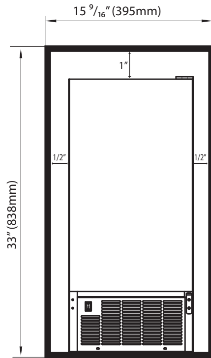
Front View
