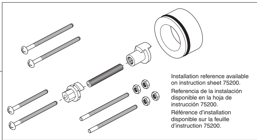
RP63696▲ Siderna™ Handle Assembly Manija Siderna™ Manette Siderna™
