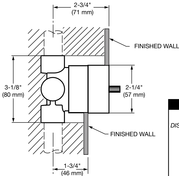
ALL CONNECTIONS 1/2" NPT
