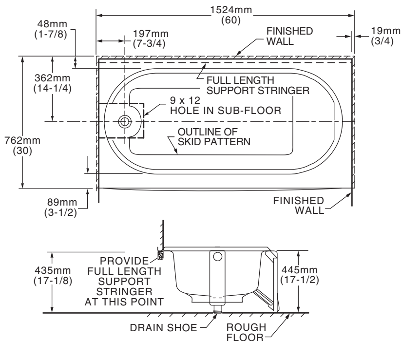
ABOVE FLOOR ROUGH 2392.202 INTEGRAL OVERFLOW 2393.202 INTEGRAL OVERFLOW
