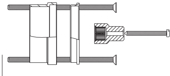
M970649-YYY0A Deep Rough-in Kit
