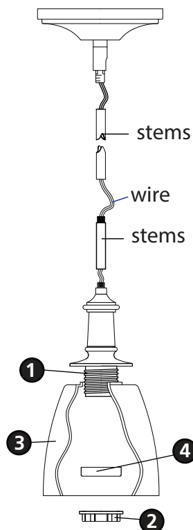
Drawing 3 - Glass Installation
