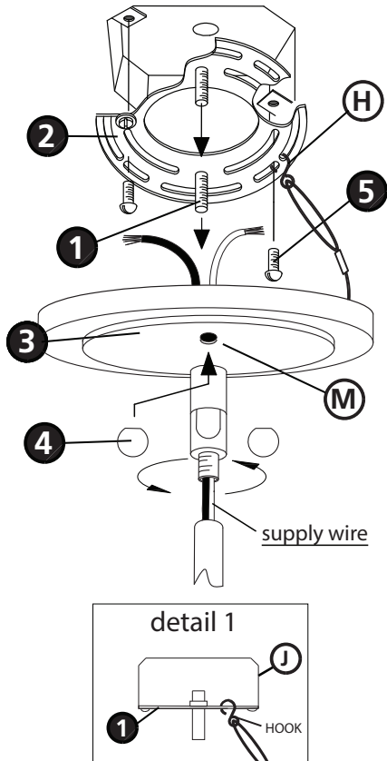
DRAWING 2 - MOUNTING
