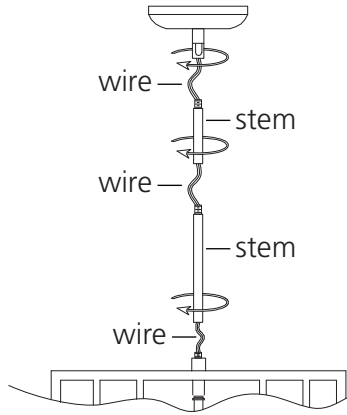
DRAWING 2 - MOUNTING
