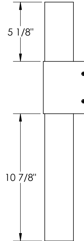
Glass Mounting Option 2
