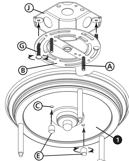
DRAWING 2 – INSTALLATION
