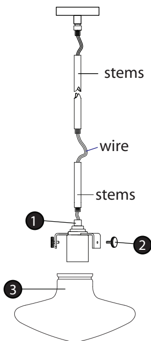
Drawing 3 - Glass Installation
