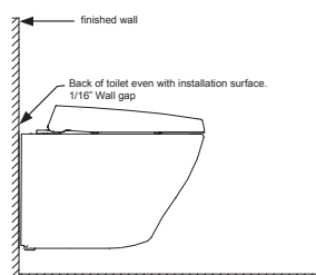
Proper Installation
